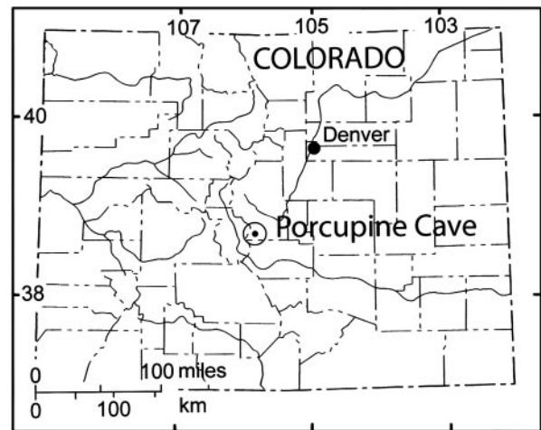
Fig. 1. Location of Porcupine Cave (small black dot) within Colorado. Circle shows 12.5-km radius around the cave. Base map is from ref. 16.
