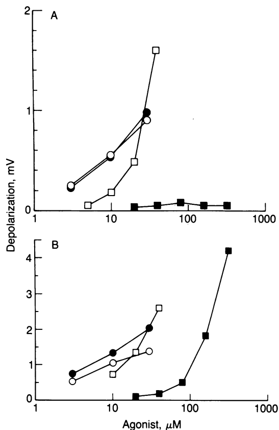
FIG. 5. Dose-response curves obtained from rat cerebral cortical slices for N -Me-D-Asp ( \square , \blacksquare ) and quisqualate ( \circ , \bullet ) before (open symbols) and following (filled symbols) 2 hr of continuous perfusion with MK-801 (235 nM, A) or phencyclidine (5 \mu M, B). MK-801 completely abolished depolarizing responses to N -Me-D-Asp but had no effect on those to quisqualate. The responses to N -Me-D-Asp were antagonized by phencyclidine and the dose-response curve was shifted to the right, whereas responses to quisqualate were slightly increased in the presence of phencyclidine.
