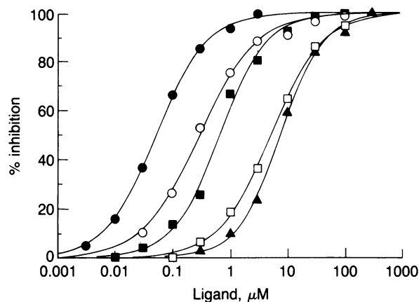
FIG. 3. Inhibition of the binding of [ ^3 H]MK-801 (5 nM) in rat cortical membranes by MK-801 (●), the (-) enantiomer of MK-801 (○), phencyclidine (■), (±)-ketamine (□), and (±)-SKF 10,047 (▲). Results are from single experiments, which were all repeated at least four times (see Table 2).
