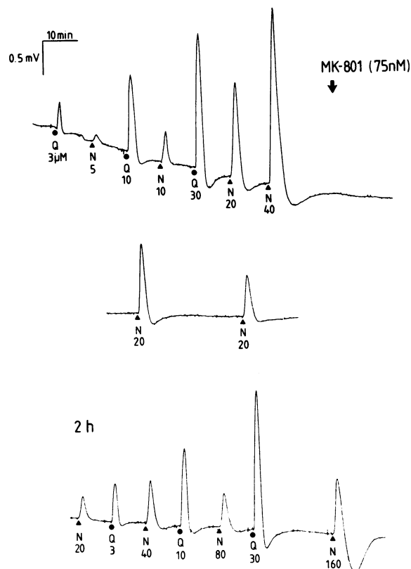
FIG. 4. Depolarizations of rat cerebral cortical tissue, relative to the white matter, produced by 1-min applications of N -Me-D-Asp (N, ▲) and quisqualate (Q, ●); the numbers indicate test concentrations in \mu M. MK-801 (75 nM) was continuously perfused from the time indicated by the arrow and N -Me-D-Asp (20 \mu M) was applied every half hour starting 1 hr later. After 2 hr of continuous perfusion with MK-801, various test concentrations of N -Me-D-Asp and quisqualate were repeated; note the insurmountable block of N -Me-D-Asp responses by MK-801.
