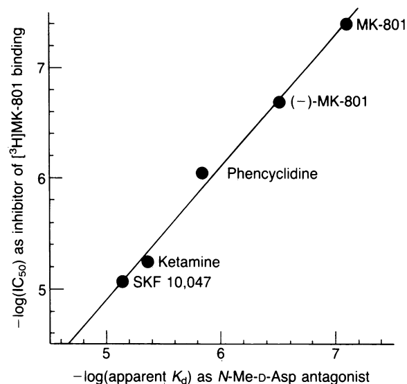
FIG. 6. Correlation between the potencies of MK-801, the ( - ) enantiomer of MK-801, phencyclidine, ( \pm )-ketamine, and ( \pm )-SKF 10,047 as inhibitors of [ ^3 H]MK-801 binding and antagonists of N -Me-D-Asp responses in the rat cortical-slice preparation. The apparent potencies for phencyclidine (5 and 10 \mu M), ( \pm )-ketamine (100 \mu M), and ( \pm )-SKF 10,047 (5 and 30 \mu M) as N -Me-D-Asp antagonists were calculated from the dose-ratios (DR) they produced at the concentrations shown, using the equation DR - 1 = B/K_d , where B is the antagonist concentration ( n = 4 or more slice preparations at each concentration). For MK-801 and its ( - ) enantiomer, the potency value was taken as the threshold dose that produced a significant reduction in N -Me-D-Asp responses, as it was impossible to estimate a dose-ratio because of the marked flattening of the dose-response relationship.
