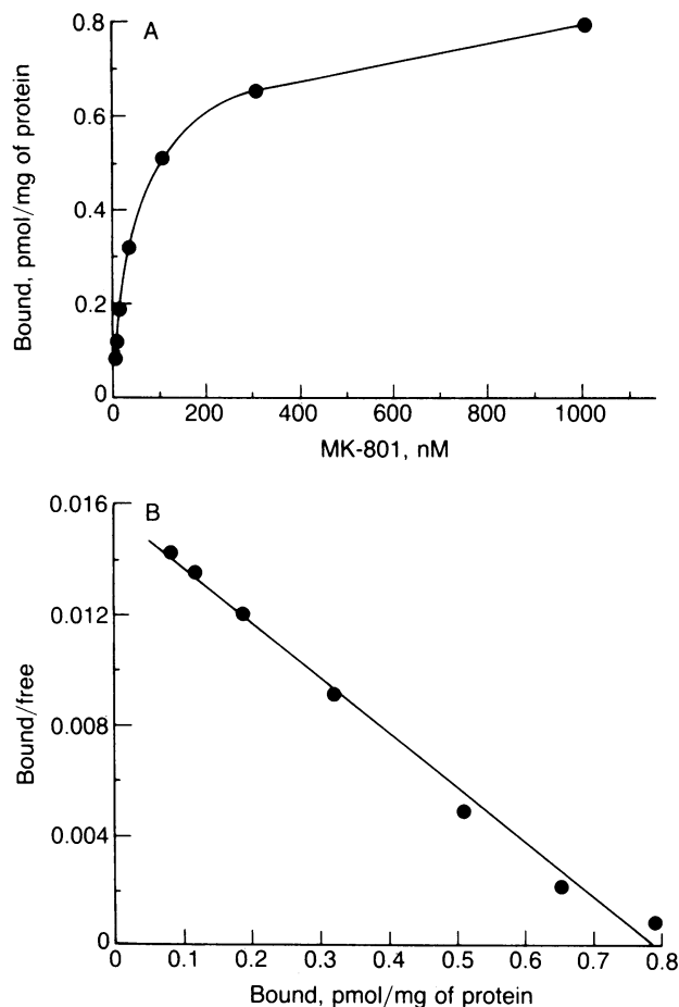
FIG. 2. (A) Saturation analysis of specific [ ^3 H]MK-801 binding to rat cortical membranes. Membranes were incubated with 5 nM [ ^3 H]MK-801 in the presence of increasing concentrations of unlabeled MK-801 (0.03–1.0 \mu M). Data are from a single experiment (which was repeated nine times, with similar results) and values are the means of triplicate determinations. (B) Scatchard plot of the specific binding data in A.
