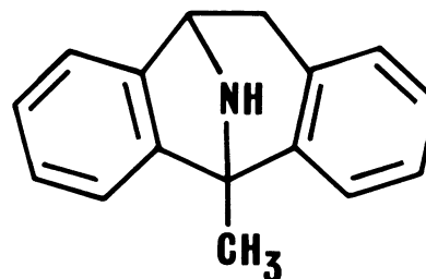
FIG. 1. Structure of MK-801, (+)-5-methyl-10,11-dihydro-5 H -dibenzo[ a,d ]cyclohepten-5,10-imine.
