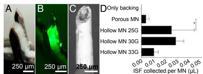
Fig. 2. ISF collection by capillary action through porous and single-capillary MNs. (A) Representative porous paper MN sandwiched between two stainless steel MNs for mechanical support (750 \mu\text{m} tall). (B) Representative porous paper MN that has absorbed ISF from pig skin soaked in fluorescein to facilitate ISF imaging. (C) Representative hollow stainless steel MN (750 \mu\text{m} tall) with a single hollow capillary to draw fluid out of skin. (D) ISF volume sampled from pig skin after 20 min: porous paper backing with no MNs (negative control), porous paper MNs, and hollow, single-capillary MNs of 33 gauge (108- \mu\text{m} i.d.), 30 gauge (159- \mu\text{m} i.d.), and 25 gauge (260- \mu\text{m} i.d.). Data show mean \pm SD ( n = 4 ); *P < 0.05 .
