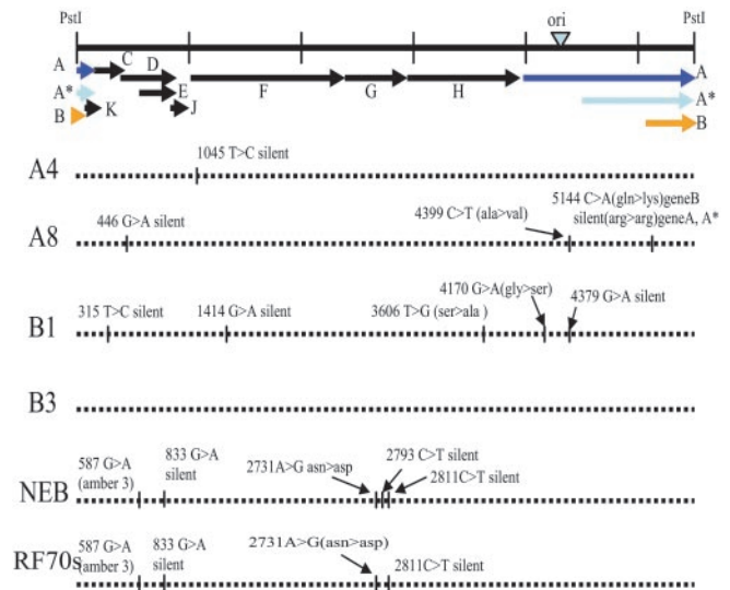
Fig. 5. Sequence comparisons of natural \phi X and syn \phi X genomes. Differences from the Sanger sequence (13) are indicated. A4, A8, B1, and B3 are the syn \phi X described in the text. NEB, \phi X RF I DNA supplied by NEB (catalog no. N30215); RF70s, DNA prepared in the late 1970s and stored since then by C.A.H.
