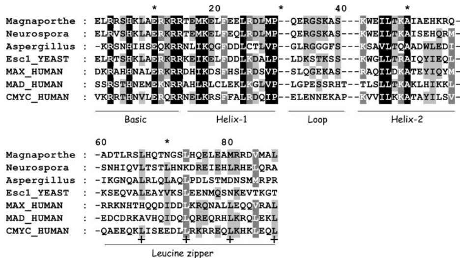
Fig. 2. Alignment of Myc, Max, and Mad together with four putative fungal Myc sequences, visualized by GENEDOC ( www.psc.edu/biomed/genedoc ), with conserved sites indicated by differential shading. Two gaps separate the various labeled functional domains. Heptad leucine repeats in the zipper are labeled with a bold plus (+) sign.
