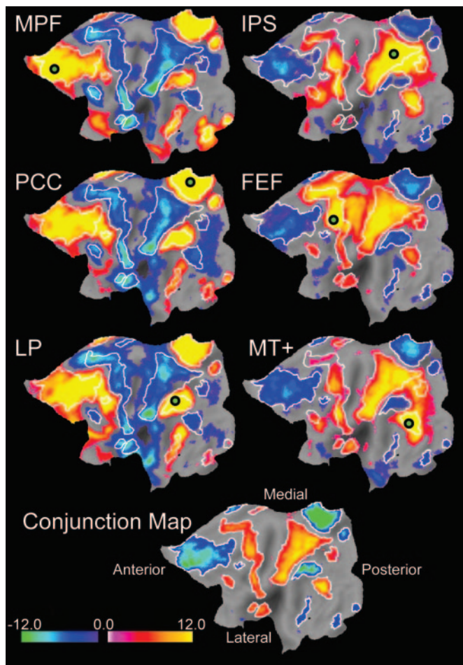
Fig. 2. Population-based z-score maps showing nodes significantly correlated or anticorrelated with six seed regions (small circles). (Upper Left) Results from three task-negative seed regions: MPF, PCC, and LP. (Right) Results from three task-positive seed regions: IPS, FEF, and MT + . (Lower) The conjunction map is an average, including only nodes significantly correlated or anticorrelated with five of the six seed regions. White contours are drawn on the conjunction map and copied onto the other maps to facilitate comparison.
