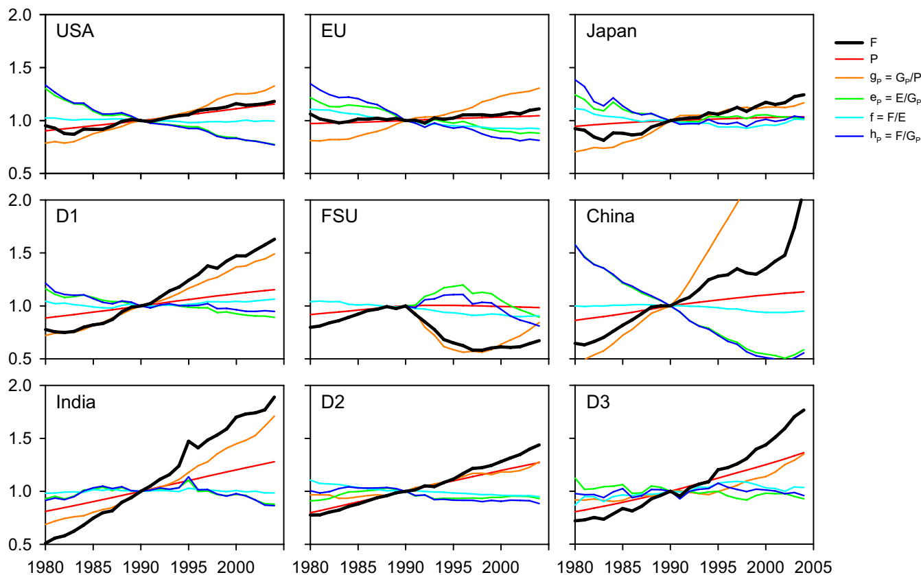
Fig. 4. Factors in the Kaya identity, F = P g e f = P g h , for nine regions. All quantities are normalized to 1 at 1990. Intensities are calculated with G_{P_i} (PPP). For FSU, normalizing G_{P_i} in 1990 was back-extrapolated. Other details are as for Fig. 2.
