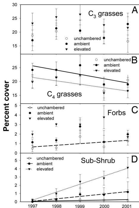
Fig. 4. Evaluations for changes in vegetative cover over 5 years of CO 2 enrichment among four functional groups: C 3 grasses (A), C 4 grasses (B), herbaceous forbs (C), and one subshrub species [ A. frigida (D)]. For each functional group, the annual mean percentage of vegetative cover was regressed on year to evaluate differences in temporal trends for plants grown under elevated (720 ppm CO 2 ) and ambient (360 ppm CO 2 ) [CO 2 ] and the unchambered control conditions in native shortgrass steppe from 1997 to 2001. Only significant ( P < 0.10 ) regressions are plotted, which include ambient ( P = 0.03 ) and elevated ( P = 0.08 ) C 4 grasses, unchambered forbs ( P = 0.04 ), and all subshrub treatments ( P < 0.0001 for elevated and ambient plots; P = 0.05 for unchambered plots). For the subshrub, slope of the elevated CO 2 line was significantly greater than slopes of the ambient CO 2 ( P = 0.006 ) and unchambered ( P = 0.001 ) lines. Each data point represents annual means from measurements taken six or seven times within each growing season; bars indicate SE.
