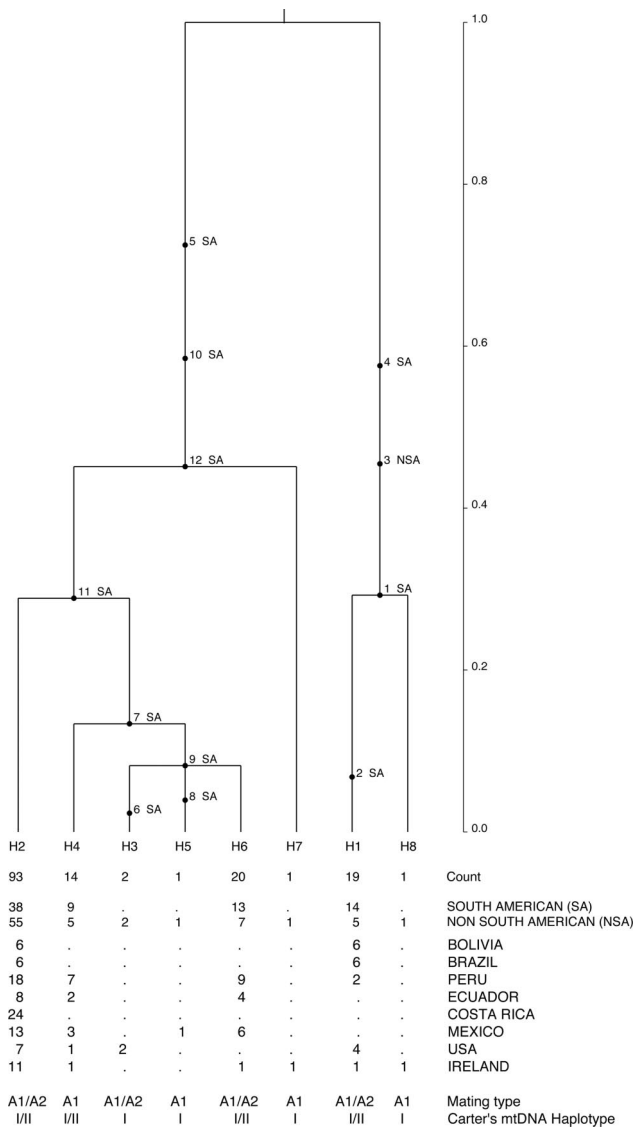
Fig. 2. The rooted coalescent-based gene genealogy showing the distribution of mutations for South American (SA: Peru, Ecuador, Bolivia, Brazil) and non-South American (NSA: Costa Rica, Mexico, U.S., Ireland) populations for the IRRAS locus of Phytophthora infestans generated using GENETREE (32). Time scale is in coalescent units of effective population size. The direction of divergence is from the top (past–oldest) to the bottom (present–youngest). The numbers below the tree from top to bottom designate each distinct haplotype and its count (i.e., the number of occurrences of the haplotype in the sample), the count of each haplotype in each population, the mating type of the isolates, and the mtDNA haplotype (33). Maximum likelihood estimates of the tree with the highest root probability, standard deviation (SD) and Watterson’s theta (55) were as follows: Likelihood = 3.5320 \times 10^{-23} , SD = 4.8689 \times 10^{-20} , theta = 2.0. Estimates were based on 10 million coalescent simulations and five independent runs to ensure convergence. Simulations were performed assuming constant population size.
