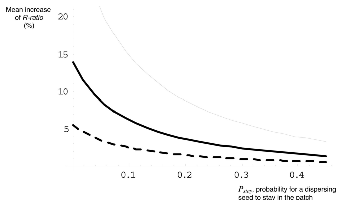
Fig. 2. Increase of the ratio of nondispersing seeds ( R -ratio) in urban patches as a function of the probability of staying within the patch, P_{\text{stay}} (see text). Results are obtained for 12 generations of selection (thin line), 5 generation of selection (thick line), and 2 generations of selection (dotted line).
