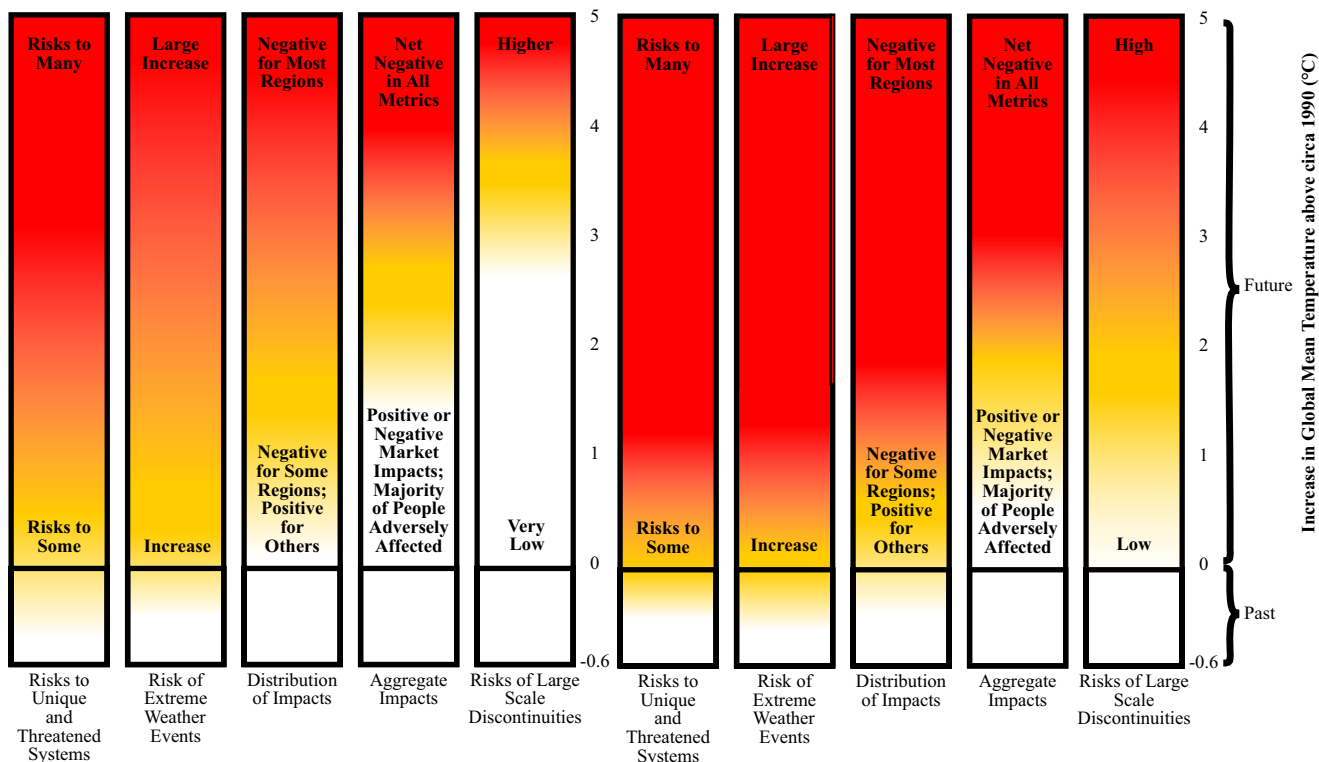
Fig. 1. Risks from climate change, by reason for concern—2001 compared with updated data. Climate change consequences are plotted against increases in global mean temperature ( ^{\circ}\text{C} ) after 1990. Each column corresponds to a specific RFC and represents additional outcomes associated with increasing global mean temperature. The color scheme represents progressively increasing levels of risk and should not be interpreted as representing “dangerous anthropogenic interference,” which is a value judgment. The historical period 1900 to 2000 warmed by \approx 0.6^{\circ}\text{C} and led to some impacts. It should be noted that this figure addresses only how risks change as global mean temperature increases, not how risks might change at different rates of warming. Furthermore, it does not address when impacts might be realized, nor does it account for the effects of different development pathways on vulnerability. (A) RFCs from the IPCC TAR as described in section 1. (B) Updated RFCs derived from IPCC AR4 as supported by the discussion in section 2. (Reproduced with permission from Climate Change 2001: Impacts, Adaptation and Vulnerability. Contribution of Working Group II to the Third Assessment Report of the Intergovernmental Panel on Climate Change. Figure SPM-2. Cambridge University Press.)
