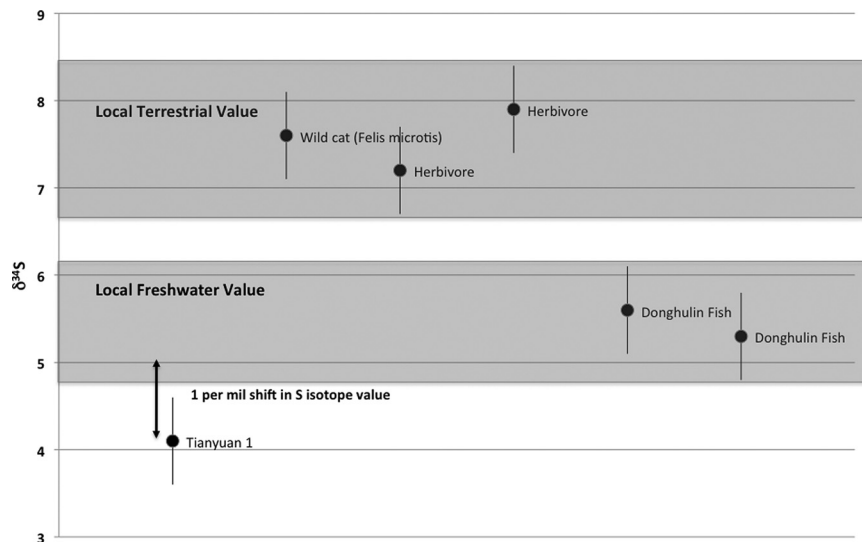
Fig. 2. Sulfur isotope values of Tianyuan 1, 3 terrestrial animals from Tianyuan Cave, and 2 fish from Donghulin. Error bars indicate measurement errors.
