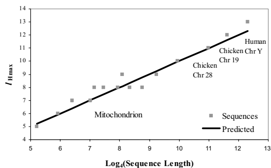
Fig. 2. Predicted vs. observed l_{Hmax} . The peak H values, or l_{Hmax} , for a sample of mitochondrial genomes and chromosomes from human and chicken were observed at different lengths, l .
