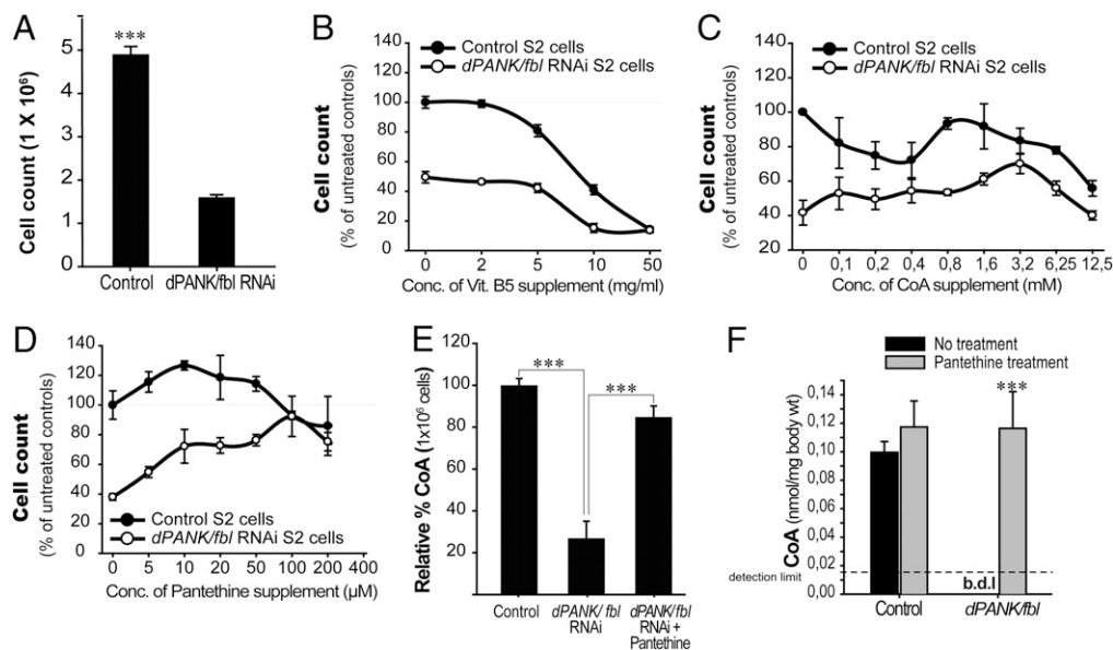
Fig. 2. Pantethine rescues cell count of dPANK/Fbl-depleted cells. (A) Control and dPANK/fbl RNAi-treated cells were counted and plated in equal numbers ( 0.35 \times 10^6 cells/mL) 4 days after dPANK/fbl RNAi treatment, and proliferation was assayed by counting cells 3 days later. ***P < 0.001 (Student's t test). Error bars indicate SEM. Control cells and dPANK/fbl RNAi-treated cells were plated, and it was tested whether VitB5 (B), CoA (C), or pantethine (D) addition to the medium rescued the cell count of dPANK/Fbl down-regulated cells. 100% represents the number of control cells under normal culturing conditions. (E) CoA levels were measured using HPLC in control cells and in dPANK/fbl RNAi-treated S2 cells (7 days after treatment) with and without addition of 100 μM pantethine. (F) HPLC was used to measure CoA levels in wild types and dPANK/fbl mutants after supplementation of 1.6 mg/mL pantethine to the food. ***P < 0.001 (Student's t test). Error bars indicate SEM. b.d.l., below detection limit.
