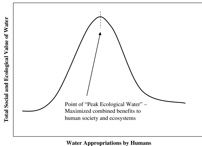
Fig. 8. This graph charts the overall value of water, a combination of social, economic, and ecological value, as water appropriation by humans increases. The value increases to a peak, where benefits to society and ecosystems is maximized, but then declines as increased appropriations lead to excessive ecosystem and social costs. Nonmonetary costs and benefits are hard to quantify, but must be included to avoid exceeding the point of peak ecological water.
