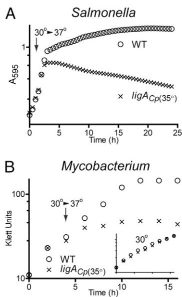
Fig. 3. Growth dependence on ligA CP renders Salmonella and Mycobacterium TS. (A) S. enterica ser. Thyphimurium with phage Mu insertion in the chromosomal ligA gene showed growth dependence on a plasmid-borne copy of ligA CP , and was TS. Half of the data-points removed for clarity. (B) M. smegmatis with a deletion of 54% of its ligA gene is supported for growth by a plasmid-borne copy of codon-optimized ligA CP .
