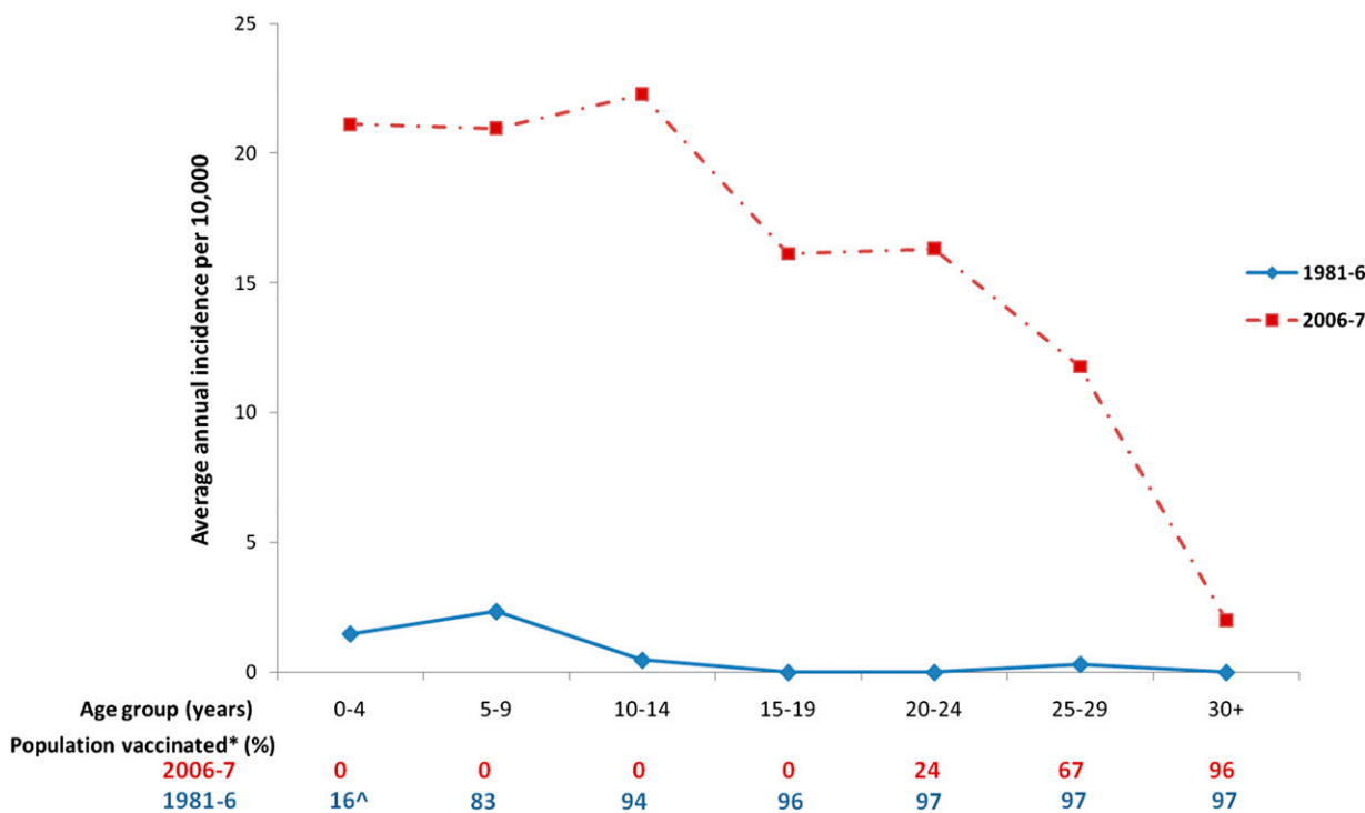
Fig. 4. Comparison of average annual cumulative incidence of human monkeypox by age group Kole Health Zone, Democratic Republic of Congo: 1981–86 vs. 2006–7. * proportion of the population vaccinated in 2006–7 and in 1981–6 based on vaccination scar surveys in 1981–6 and in 2006. ^ , vaccination rate steadily declined from 41.0% in 1981 to 4% in 1985 (13, 33).
