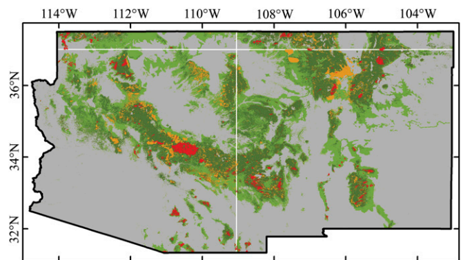
Fig. 5. Map of SW forest and woodland mortality due to bark beetles from 1997 to 2008 (orange) and wildfire (red) from 1984 to 2006. Dark green areas are conifer and mixed forest. Light green areas are piñon/juniper woodland. Gray areas are nonforest or hardwood/shrub woodland landscapes. White lines are state boundaries. Bark-beetle-induced mortality covered 18,177 km 2 , and wildfire induced mortality covered 6,420 km 2 .
