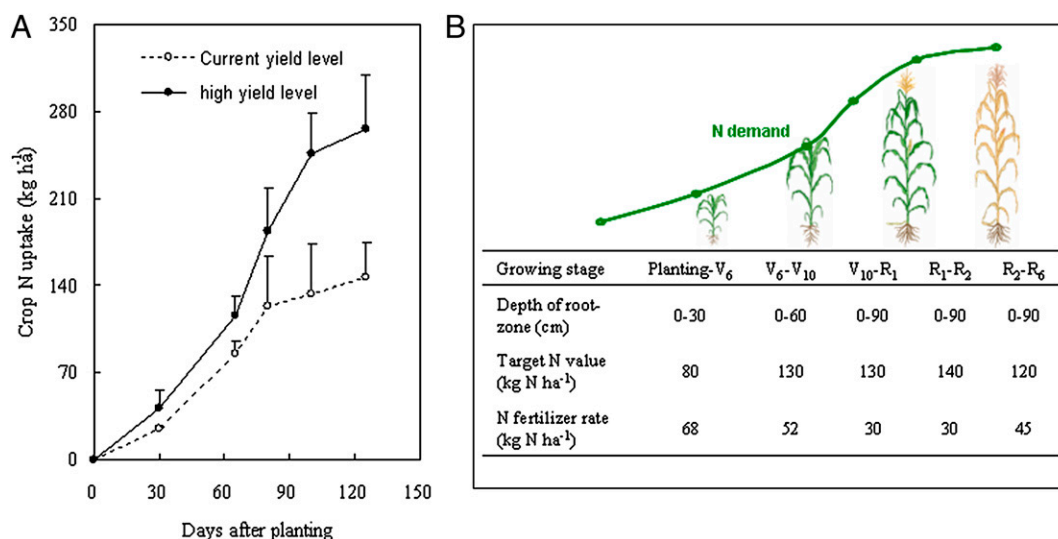
Fig. 4. (A) Timing of N uptake by maize grown with current farmers' practice (average yield, 6.4 t ha -1 , n = 22) and with the cropping system designed using the hybrid maize model (Fig. 3) (with an average yield of 13.1 t ha -1 , n = 27). (B) Target N value in the root zone, and the actual N fertilizer application required to meet the target values calculated using the IRNM system for maize with a high yield level of 13 t ha -1 . Through IRNM, the growth season of maize was divided into five periods (34). The target N value was the sum of N uptake by shoot and root scaled by target yield and the needed minimum residual of soil available N at the end of each growth period (32, 33). The optimal rate of N fertilizer application in each maize growth period was determined by deducting measured soil nitrate-N content in root zone from the target N value.
