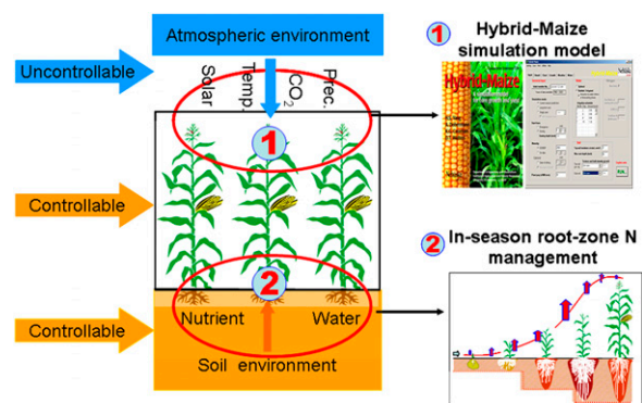
Fig. 2. Conceptual framework for the ISSM approach. Blue arrow represents the atmospheric environment, including solar radiation, temperature, precipitation, and CO 2 concentration—all factors that agricultural practices cannot control but must adapt to. Orange arrows represent crop canopy and soil nutrient or water supply, which can be altered by agricultural practices. Using the Hybrid-Maize model (29) (Upper Right), we selected the most appropriate combination of planting date, crop maturity, and crop variety to optimize capture of radiation and favorable growing conditions at a given site. Using an IRNM strategy (32, 33) (Lower Right), we managed total N supply to match high-yielding crop N requirements in time, space, and quantity.
