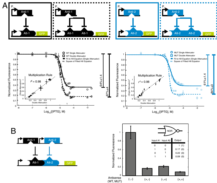
Fig. 4. Increasing attenuation and logically controlling expression with attenuators in tandem. (A) Induction curves using an IPTG-inducible P_{\text{LacO-1}} promoter (28) (P) for single (circles; solid lines) and double (squares; dashed lines) attenuators in series. The wild-type (black) and mutant (blue) composite attenuators show similar attenuation over the full range of induction. Measured fluorescence was normalized to the case with [\text{IPTG}] = 0 \text{ mM} for each attenuator (MEFL: single WT 12725, double WT 5744, single MT 14561, double MT 5348). Hill equation fits to the single attenuator data are in solid curves. The dotted lines were calculated by squaring the fitted Hill functions (see SI Appendix ). (Insets) Plots show the comparison between the measured double attenuation and the square of measured single attenuation (calculated as 1 - \text{normalized fluorescence} ) to verify the multiplication model. Error bars represent the difference between measurements on two independent transformants. (B) Composed orthogonal attenuators have a NOR logical expression pattern. Data were normalized to 1 for the no antisense condition. Error bars represent the standard deviation from measurements on at least three independent transformants. (Inset) Table shows the measured performance of the NOR logical gate, and the expected values for a perfect digital NOR gate (parentheses).
