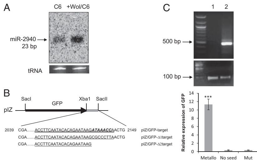
Fig. 4. Target validation of aae-miR-2940. (A) Northern blot analysis of expression of aae-miR-2940 in Wolbachia -infected C6/36.wMelPop-CLA (+Wol/C6) and uninfected C6/36 (C6) cells. (B) Cloning strategy of the metalloprotease (metallo) target, mutated target, and target with deleted sequences complementary to the miRNA seed region from the metalloprotease 3'UTR under the GFP reporter gene ORF in the pIZ vector, denoted as pIZ/GFP target, pIZ/GFP-Δ1 target, and pIZ/GFP-Δ2 target constructs, respectively. Constructs were transfected into C6/36.wMelPop-CLA cells that overexpress aae-miR-2940. RT-qPCR analysis indicated that GFP expression was significantly higher ( P < 0.0001 ) in pIZ/GFP-target (metallo) transfected cells than in pIZ/GFP-Δ1target (mut) and pIZ/GFP-Δ2target (no seed) transfected cells. Target sequences are underlined, and seed region complementary sequences are shown in bold italic type. (C) RT-PCR analysis of metalloprotease gene expression in Aag2.wMelPop-CLA cells at 48 h posttransfection with a synthetic inhibitor of aae-miR-2940 (1) and a control inhibitor with random sequences (2). Actin gene expression was analyzed in both experiments as a loading control.
