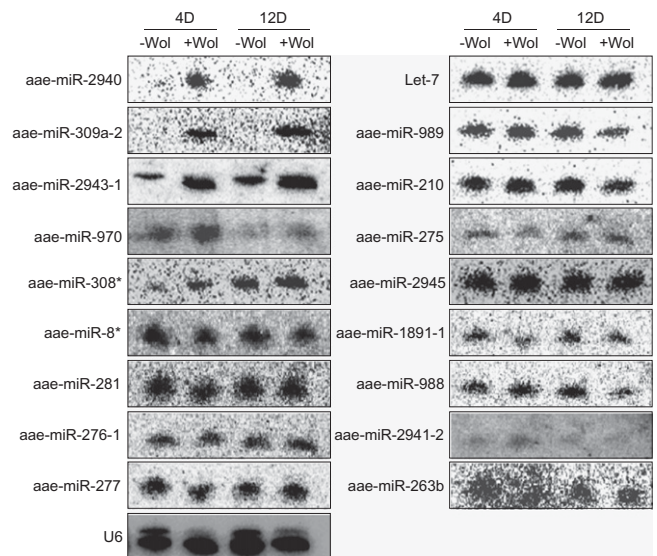
Fig. 2. Validation of expression profile of miRNAs differentially expressed in mosquitoes. Aae-miRs that were significantly up-regulated or down-regulated in Wolbachia -infected (+Wol) and uninfected (-Wol) 4-d-old and 12 d-old females were analyzed by Northern hybridization with probes specific to each miRNA. The same blot was used multiple times after removal of probes. U6 was used as a control to demonstrate equal loading of samples.
