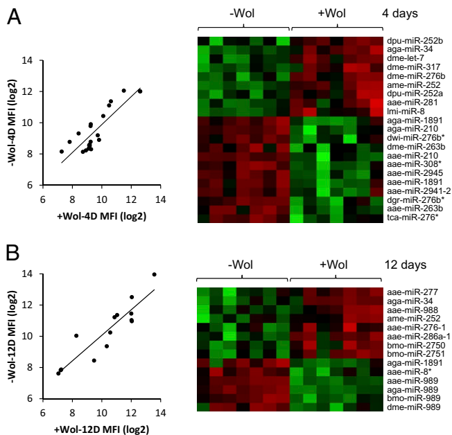
Fig. 1. Wolbachia infection alters adult mosquito cellular miRNA expression profile, as determined using microarrays. Expression profiles of miRNAs that were significantly up or down-regulated in 4-d-old (A) and 12-d-old (B) Wolbachia -infected female Ae. aegypti (+Wol) compared with uninfected (-Wol) female mosquitoes are shown. MFI, mean fluorescent intensity. The corresponding miRNA microarray color map shows expression levels of insect miRNAs in -Wol and +Wol samples. Each miRNA was replicated seven times on each chip. Red and green indicate up-regulation and down-regulation of expression, respectively.
