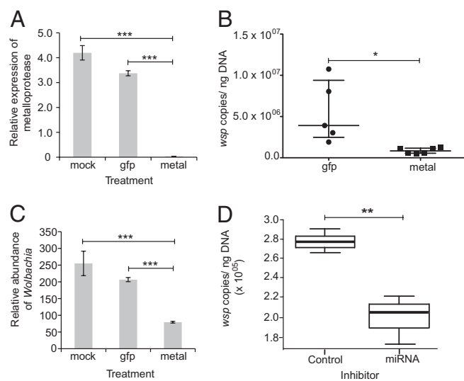
Fig. 5. RNAi-mediated silencing of the metalloprotease gene. (A) RT-qPCR analysis of the metalloprotease gene relative to actin in Aag2.wMelPop-CLA cells 48 h after transfection with mock, GFP, and metalloprotease (metal) dsRNAs. Three biological replicates were analyzed for each transfection. Asterisks indicate a significant difference between transfection with metalloprotease dsRNA and the other treatments ( P < 0.0001 ; t test). (B) Differences in the density of Wolbachia in Aag2.wMelPop-CLA cells transfected with the metalloprotease (MP) and GFP dsRNAs examined by qPCR ( P = 0.0415 ; t test). (C) Differences in the density of Wolbachia in +Wol adult mosquitoes injected with sterile water, GFP and the metalloprotease (metal) dsRNAs, analyzed using qPCR. Five biological replicates were analyzed per injection type. Asterisks indicate significant difference between mosquitoes injected with metalloprotease dsRNA and the other treatments ( P < 0.0001 ; t test). (D) A significant difference in the density of Wolbachia in Aag2.wMelPop-CLA cells transfected with aae-miR-2940 inhibitor versus control inhibitor (random sequence) ( P < 0.0001 ; t test), analyzed by qPCR. Three biological replicates were analyzed for each transfection.
