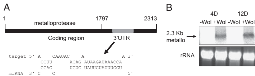
Fig. 3. Aae-miR-2940 target prediction and expression levels of the corresponding target. (A) The Ae. aegypti metalloprotease gene was predicted to be the best target with complete seed region (underlined) complementarities. The target sequence was identified in the 3'UTR of the metalloprotease gene. (B) Northern blot analysis of total RNA extracted from Wolbachia -infected (+Wol) and uninfected (–Wol) female Ae. aegypti at 4 d and 12 d after emergence. The blot was hybridized with a probe specific to the metalloprotease (metallo) gene. rRNA is shown to indicate equal loading of samples.
