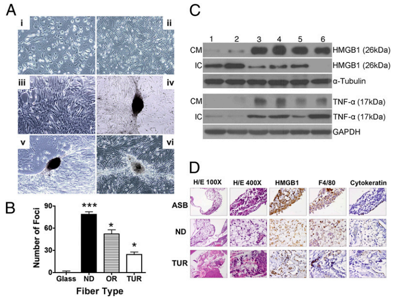
cells in culture, that asbestos and erionite can cause focus formation (22). However, the same fibers can cause MM in animals. Thus, it is believed that the chronic inflammatory process and consequent release of HMGB1 and TNF- \alpha over the course of years, and possibly the effect of other cofactors and cocarcinogens, are required to promote the accumulation of genetic damage that leads to the development of an immortal malignant clone. Therefore, the finding that ND erionite caused a larger number of foci to be formed in vitro than Turkish erionite should not be taken independently as evidence that ND erionite is more potent than Turkish erionite, because carcinogenesis is a much more complex phenomenon (27). However, focus formation is evidence that these two types of erionite have similar biological effects on human mesothelial cells.
