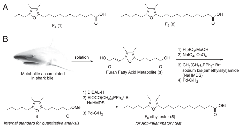
Fig. 1. (A) Structures of the representative furan fatty acids detected in the green-lipped mussel. (B) Partial synthesis of furan fatty acid F_6 .
