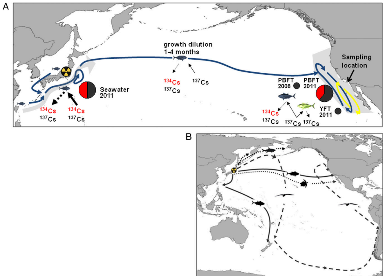
Fig. 1. (A) Map of the northern Pacific ocean showing simplified movement patterns for juvenile PBFT (blue arrows) from Japan to the CCLME and juvenile YFT (yellow arrows) in the CCLME. Kuroshio Current (gray arrow east of Japan) and CCLME (gray region west of N. America) are shown. Pie charts show mean concentrations of ^{134}\text{Cs} (red) and ^{137}\text{Cs} (dark gray) in seawater ( \text{Bq m}^{-3} ) (3), and muscle tissue ( \text{Bq kg}^{-1} ) in PBFT after Fukushima, PBFT before Fukushima, and YFT after Fukushima. Pie charts for fish are sized to scale of total radiocesium concentrations. Black arrows show uptake (solid arrows) and efflux (dotted arrows) of radiocesium in different ocean regions (arrow thickness scaled for relative efflux and uptake rates). (B) Simplified migration patterns of some highly migratory species in the Pacific that inhabit waters around Japan and make subsequent long distance migrations to distant ecoregions including Kamchatka, the Aleutian Islands, North America, South America, and New Zealand. Migration patterns are shown for salmon sharks (17) (short dashed line), sooty shearwaters (18) (long dashed line), Pacific bluefin tuna (6) (solid lines), and loggerhead turtles (19) (dotted line).
