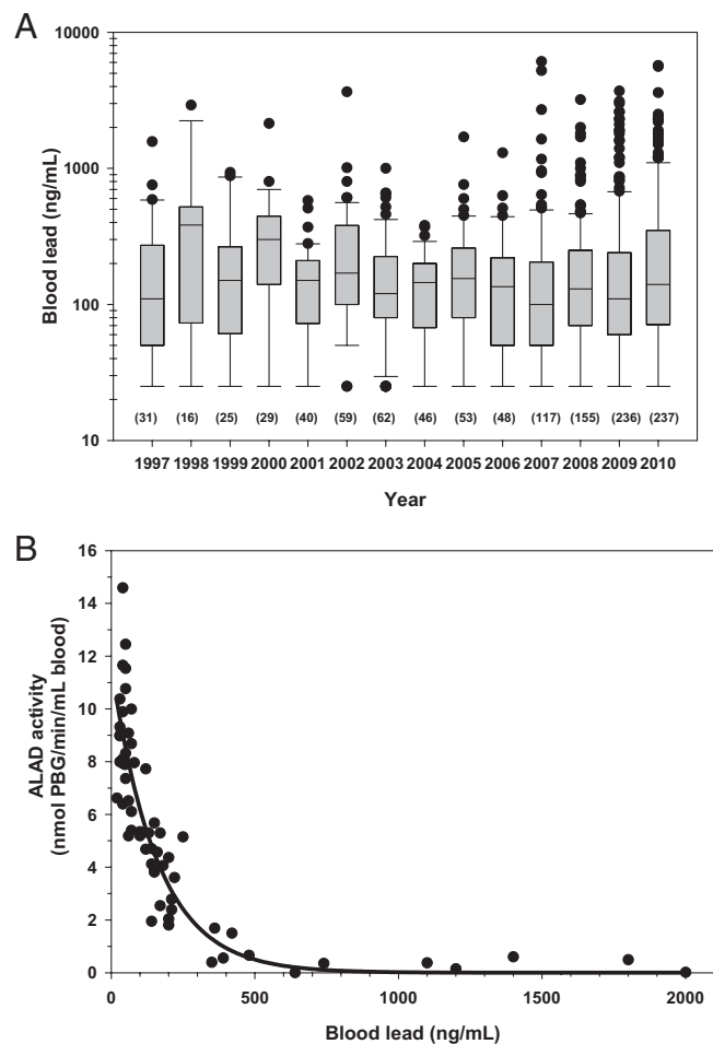
Fig. 2. California condor blood lead levels and sublethal exposure effects show that the population is negatively impacted by chronic lead exposure. (A) Blood lead levels of condors in California by year. Box indicates median, upper and lower bounds are 75th and 25th percentiles, whiskers represent 10th and 90th percentiles, (number of samples), y axis is log scale, lowest value presented is 25 ng/mL (one-half the measurement detection limit). (B) ALAD activity vs. blood lead levels in free-flying condors in California. Data show that there is a significant decreasing exponential relationship between blood ALAD activity and blood lead level [the equation is ALAD activity (nanomoles porphobilinogen per minute per milliliter blood) = 11.6 \times e^{(-0.006 \times \text{blood lead in nanograms per milliliter})} , R = 0.891 , P < 0.001 , n = 60 ].
