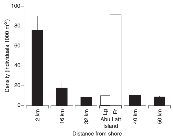
Fig. 2. Underwater visual census estimates. Adult L. ehenbergii densities (mean \pm SD) on reefs at five distances offshore ( n = 2 reefs per distance) and two habitats at Abu Latt Island (24-km offshore). Fr, fringing reef habitat; Lg, lagoon habitat.
