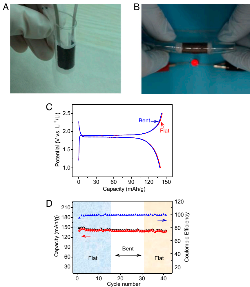
Fig. 4. Characterization of a thin, lightweight, and flexible LTO/GF/LFP/GF full battery. (A) Photograph of a bent battery encapsulated by PDMS, showing its good flexibility. (B) Lighting a red LED device under bending. (C) Galvanostatic charging/discharging curves of the battery. Red and blue lines represent the as-fabricated flat battery and the bent battery after repeatedly bending to a radius of 5 mm 20 times, respectively. (D) Cyclic performance of the battery under flat and bent states.
