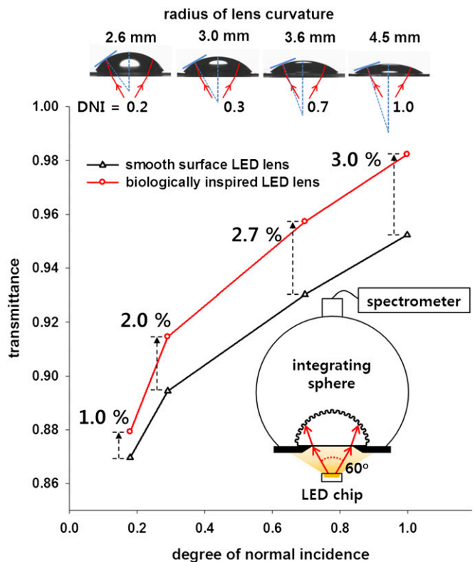
Fig. 4. Light transmission through the biologically inspired LED lens depending on lens curvatures under a constant LED emitting angle of \pm 30^\circ . DNI, the ratio of a near normal incidence angle to lens surface over total emitting angle of an LED light source, increases with the ROC. The biologically inspired LED lens shows the maximum transmission at DNI = 1.0; that is, the lens surface has near normal incidence for all rays from an LED light source (also corresponds to the LED lens of 4.5 mm in ROC).
