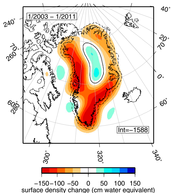
Fig. 2. Geographical pattern of the ice mass change over Greenland averaged for the period between January of 2003 and January of 2011. The map is the result of the combination of signal estimates conducted on individual time series of Slepian function expansion coefficients. The integral value (Int) for the entire epoch is shown in gigatons. The 0-cm water contour is shown in black.
