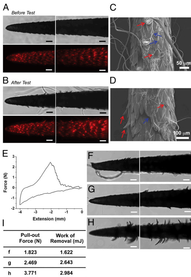
Fig. 5. Generation of mechanical adhesion by microstructured barbs. (A and B) Representative optical and fluorescent images of porcupine quills before and after removal from porcine skin. Fluorescence images are useful to delineate the boundaries of individual barbs and are obtained by merging several images taken at different focal planes along the z axis. (Scale bar: 100 \mu\text{m} .) (C and D) FE-SEM micrographs following removal of quills from porcine skin. Residual tissue is indicated by blue arrows. Red arrows in figures indicate bending of barbs during pull-out. (E) A representative force versus extension plot for a penetrating depth of 4 mm where puncture typically occurs following tissue compression of 1–2 mm ( n = 5 ). (F–H) Images of quills following removal from porcine skin are useful to examine the heterogeneity of tissue interactions and to establish the relationship between the bending of barbs and relative level of tissue adhesion summarized in the table (I). (Scale bars: 100 \mu\text{m} .) See Fig. S3A for the experimental set-up for the tests with porcine skin.
