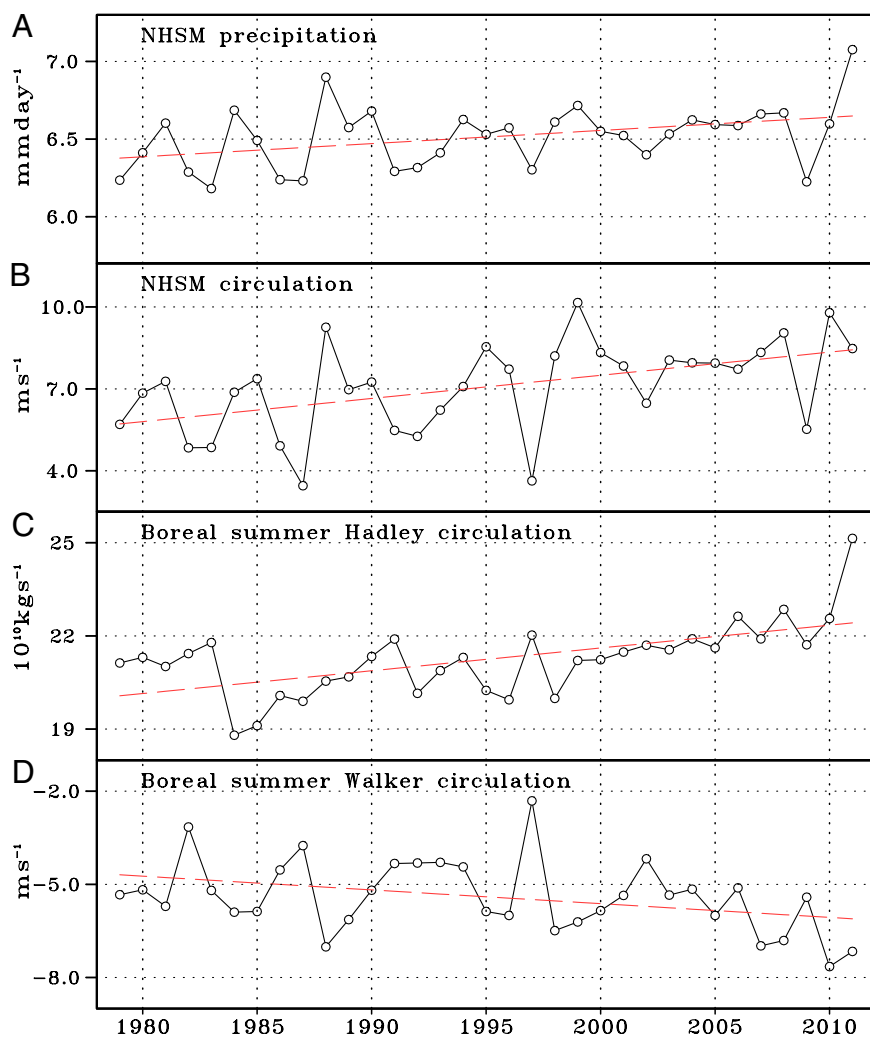
Fig. 2. Variability and trends of the NHSM system, and the Hadley and Walker circulation. Time series of boreal summer (MJAS) mean indices representing (A) NHSM precipitation intensity ( \text{mm}\cdot\text{d}^{-1} ) averaged over the entire NH monsoon rainfall domain; (B) NHSM circulation intensity measured by the vertical shear of zonal wind (850 hPa minus 200 hPa) averaged over 0^{\circ}\text{--}20^{\circ}\text{N} , 120^{\circ}\text{W}\text{--}120^{\circ}\text{E} , which significantly correlates with the NHSM's precipitation index ( r = 0.85 ); (C) Hadley circulation intensity measured by the maximum absolute value of the cross-equatorial, zonal mean meridional mass stream function ( 10^{10} \text{ kg}\cdot\text{s}^{-1} ); and (D) Walker circulation intensity measured by the low-level zonal winds at 850 hPa averaged over the equatorial Pacific ( 10^{\circ}\text{S}\text{--}10^{\circ}\text{N} , 140^{\circ}\text{E}\text{--}120^{\circ}\text{W} ). The red dashed lines in each panel denote the linear trends, and their statistical significances are shown in Table 1. The ERAI and GPCP, version 2.2, data were used for the period of 1979–2011.
