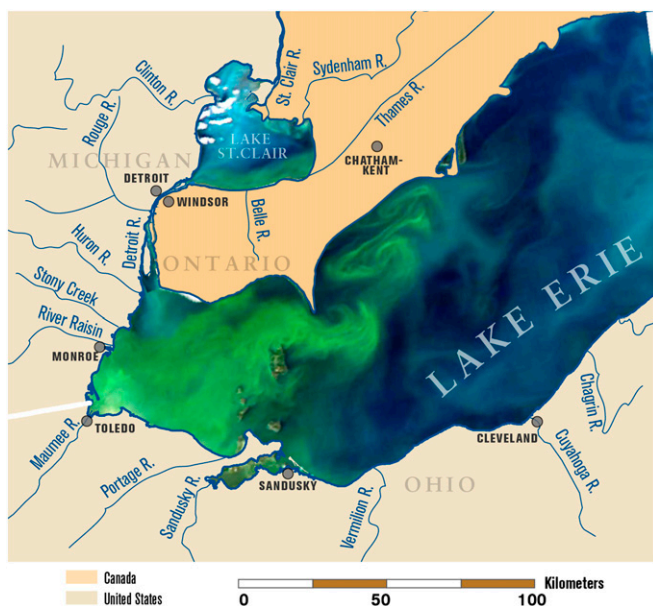
Fig. 1. MODIS satellite Image of Lake Erie on September 3, 2011, overlaid over map of Lake Erie tributaries. This image shows the bloom about 6 wk after its initiation in the western basin. On this date, it covers the entire western basin and is beginning to expand into the central basin, where it will continue to grow until October (Fig. S1).
