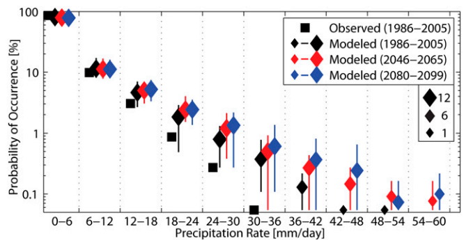
Fig. 4. Probability of daily precipitation intensities for spring (March–April–May) averaged over the western Lake Erie basin (40–43°N, 82–85.5°W) as observed by the Climate Prediction Center (CPC) gridded data (black squares) for the present-day time period (1986–2005), as modeled by a 12-model multimodel average for the same present-day time period (black diamonds) and for two future time periods of 2046–2065 (red diamonds) and 2080–2099 (blue diamonds). Vertical lines represent the range of individual model predictions for those models with a nonzero probability of a given event size. Diamond size represents the number of models included in each calculation (i.e., the number of models with nonzero probabilities for a given event size), ranging from 0 to 12. Individual model members are shown in Fig. S9.
