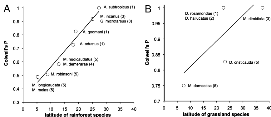
Fig. 1. Mean index of seasonal predictability in arthropod abundance (Colwell's P) plotted against mean latitude of sample points for 10 species of dasyurid and didelphid marsupials in rainforest habitats (A) and 5 species in grassland (B). P = 1 if there is complete between-year predictability in the months of peak arthropod abundance. Numbers in parentheses are ranks of iteroparity in males: (1) die-off, (2) facultative semelparity, (3) <1\% survival between cohorts, no die-off, (4) 1–10% survival between cohorts, (5) iteroparity.
