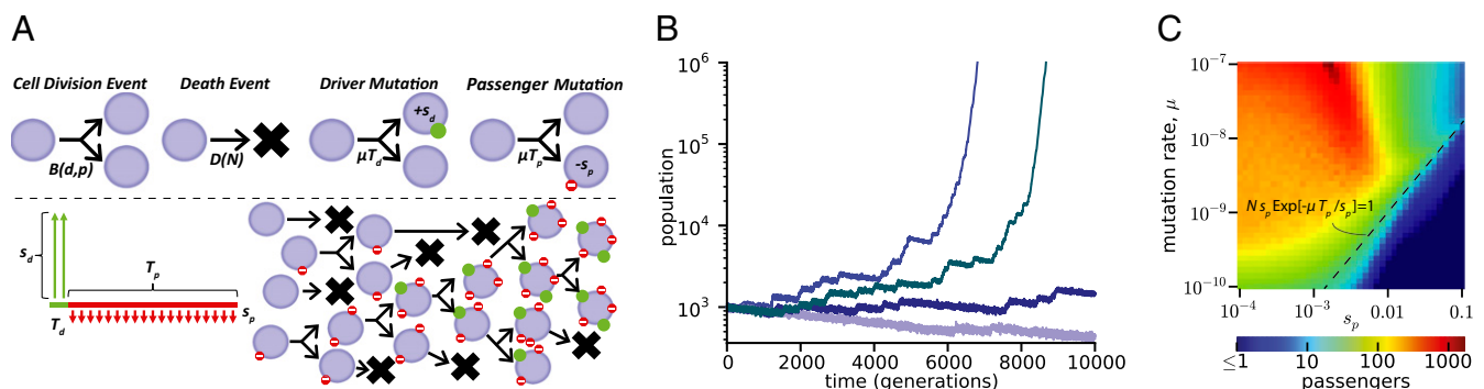
Fig. 1. Dynamics of cancer progression. (A) Our evolutionary model: individual cancer cells stochastically divide (potentially acquiring new drivers/passengers) and die. A new driver increases the birth rate by s_d , whereas a passenger decreases it by s_p (Eq. 1). Drivers arise rarely, but have large effects, while passengers are common, but have small individual effects. (B) Simulated cancer progression using a Gompertz death rate; despite identical parameters, trajectories exhibit markedly different behavior, sometimes regressing to extinction or having long periods of dormancy. (C) The number of accumulated passengers increases with mutation rate and depends, nonmonotonically, on passenger strength.
