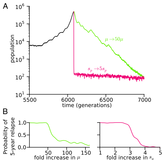
Fig. 5. Deleterious passengers can be exploited for treatment. (A) Cancers grown to 10^6 cells are treated by increasing the mutation rate (green) or deleterious effect of passengers (magenta). Both strategies lead to reduction in cancer size. (B) Much smaller increase of the deleterious effect of passengers is sufficient to prevent 5-y relapse.
