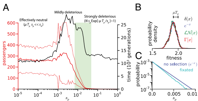
Fig. 3. Moderately deleterious passengers alter cancer progression and mostly evade selection. (A) Passengers of intermediate fitness effect s_p prolong the time to cancer and accumulate in large, highly variable quantities (red solid, mean; dotted, \pm 1 SD). Moderately deleterious passengers affect cancer only if they are strong or frequent enough to be comparable to the effects of drivers, yet weak enough to avoid selection (SI Appendix, SI Text). Experimentally observed fitness effects of random point mutations in YFP in yeast ranged from 0.007 to 0.028 (green shading) (14). (B) Population dynamics did not change noticeably when passengers were drawn from various distributions of fitness distributions (SI Appendix, SI Text). (C) Passenger fixation probability declined only moderately with increasing deleteriousness.
