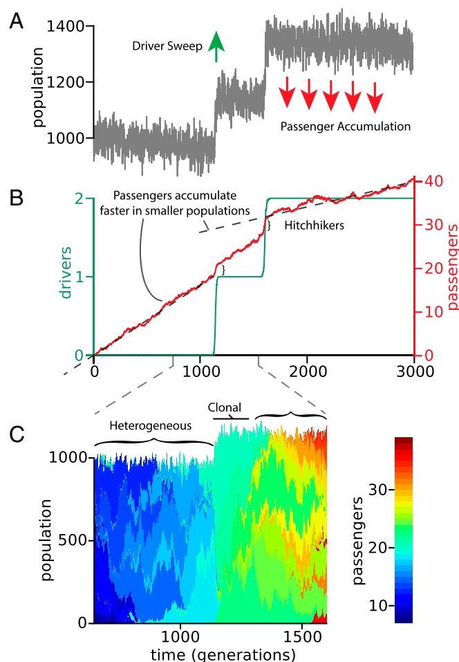
Fig. 2. Mechanisms of passenger accumulation. (A) Spurts of population growth, caused by the acquisition of a new driver, are interspersed with a gradual decline due to passenger accumulation. (B) Passengers accumulate both steadily between the arrival of drivers and by hitchhiking during clonal expansions. (C) Each subclone, containing a unique number of passengers (shown by color), grows and declines stochastically, eventually to extinction. In between drivers, the population becomes heterogeneous. A new driver will promote only one clone, creating a clonal population. Afterward, new mutations on top of the previous hitchhikers restore heterogeneity.
