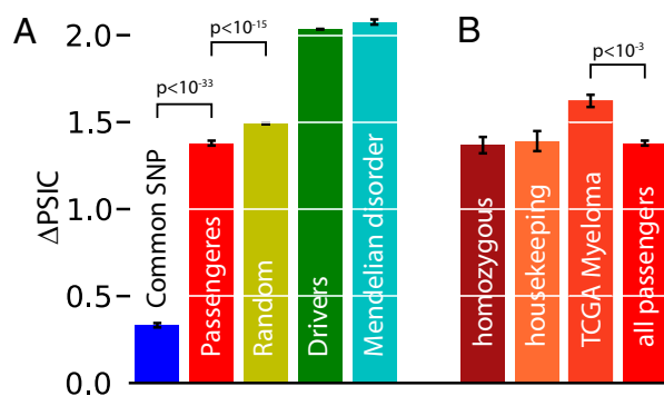
Fig. 4. Characterization of missense mutations in cancer sequencing data. (A) Mutations were assayed using the \Delta PSIC score of PolyPhen, which estimates the damaging effect of a new mutation, given known homologs; mutations with high \Delta PSIC scores are most likely damaging (43). Passengers have large \Delta PSIC , close to random mutations, suggesting that they are deleterious. (B) Deleterious passenger phenotypes were observed in all subsets of passengers studied, arguing that these results cannot be explained by recessive phenotypes, or lack of expression, or database biases.
