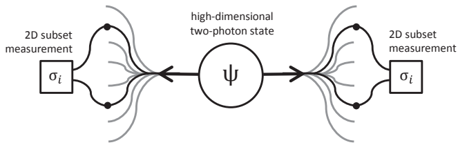
Fig. 1. Visualization of the measurement concept. The two photons are sent in two different directions. Each of the photons is in a mixture of many modes. We perform the same two-dimensional subspace measurement on both photons. When we consider all two-dimensional subspaces, we can determine the dimensionality of entanglement.
