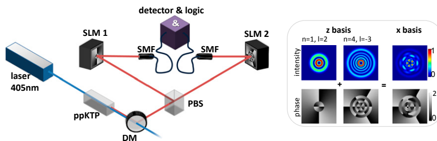
Fig. 2. (A) Schematic of the experimental setup. We pump a type-II nonlinear periodically poled potassium titanyl phosphate (ppKTP) crystal with a 405-nm, ~40-mW single-mode laser. SPDC creates collinear photon pairs with 810-nm wavelength and orthogonal polarizations. We remove the pump beam at a dichroic mirror (DM) and separate the two photons at a polarizing beam splitter (PBS). In both arms of the setup we use SLMs to perform a mode transformation of the photons. The transformation done by a computer-generated hologram at the SLM converts a specific mode into the fundamental Gauss mode. Only the Gauss mode couples into an SMF, thus the SLM + SMF combination acts as a mode filter (39). In the end, we detect the photons with avalanche photodiode based single-photon detectors and analyze the time correlation using a coincidence logic. (B) An example of a two-dimensional subspace is shown. The intensities and phases for two different modes in the z basis are demonstrated, and their superposition leads to a mode in the x basis. The y basis can be constructed similarly.
