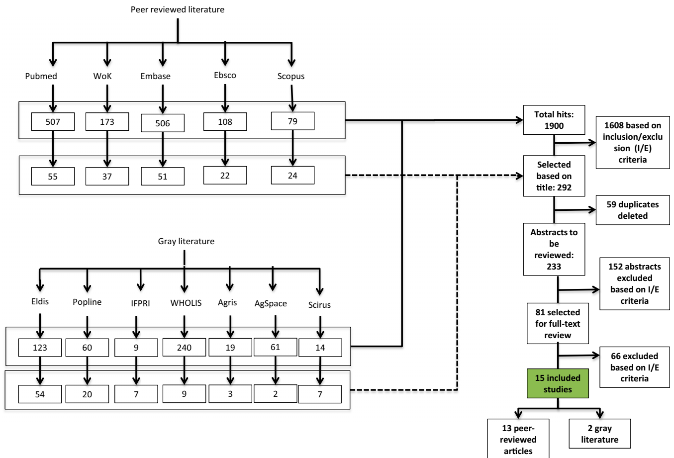
Fig. 1. Decision tree for article exclusion/inclusion.
