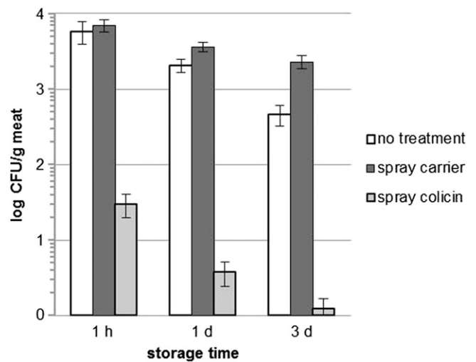
Fig. 3. Reduction of bacterial populations of E. coli O157:H7 (strain DSM19206) on fresh steak meat by colicins. Bacterial populations recovered from steak meat upon storage for various periods of time at 10 °C upon colicin treatment (colM + colE7 at 3 + 1 mg/kg meat, respectively) of contaminated meat by spray application. Error bars indicate SD of biological replicates ( n = 4 ).
