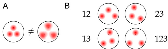
Fig. 2. (A) Observed distribution shows no displacement of the beams, whereas naively we would expect the beam to be moved and deformed, due to a combination of different cases depicted in B, which depend on which particles are in the same arm and repel each other.
