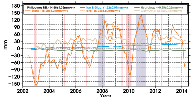
Fig. 3. Time-variable sea-level contributions to the east of the Philippines. Warm (El Niño, red) and cold (La Niña, blue) phases are highlighted whenever the MEI gets larger than 1 or smaller than -1 , respectively. The asterisk indicates that the trend is computed over the period where there are Ishii data available (2002–2012). Plots of other regions can be found in the SI Appendix .
