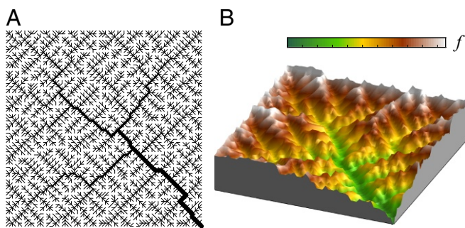
Fig. 4. OCN and landscapes. (A) An OCN derived within a 64 \times 64 regular 2D lattice by means of a simulated annealing approach ( SI Appendix ) assuming \gamma = 1/2 . The algorithm ensures that the state is a local, dynamically accessible minimum, not necessarily the absolute minimum of the function \mathcal{E}_\gamma(T) . (B) The corresponding landscape (i.e., the elevation h_v ) computed assuming \Delta h_v \propto A_v(T)^{-1/2} . We have verified numerically that the obtained OCN is a natural river spanning tree.
