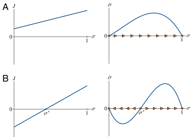
Fig. 1. Population dynamics of a scientific field, depending on its power ( 1 - \beta ), significance ( \alpha ), and homophilous bias ( \epsilon ). (A and B, Left) Graphs display [2], which relates the Youden index ( J ) to the share of Better scientists in the tenured population ( \sigma ). (A and B, Right) Graphs are phase lines for [5], which describes how the share of Better scientists ( \sigma ) evolves over time. (A) High power: 1 - \beta \geq \alpha + \epsilon/(1 + \epsilon) . When a science has high power, the Better paradigm necessarily prevails. (B) Low power: 1 - \beta < \alpha + \epsilon/(1 + \epsilon) . When a science has low power, the Worse paradigm may prevail; this happens when many scientists initially believe in the Worse paradigm [ \sigma(0) < \sigma^* ].
