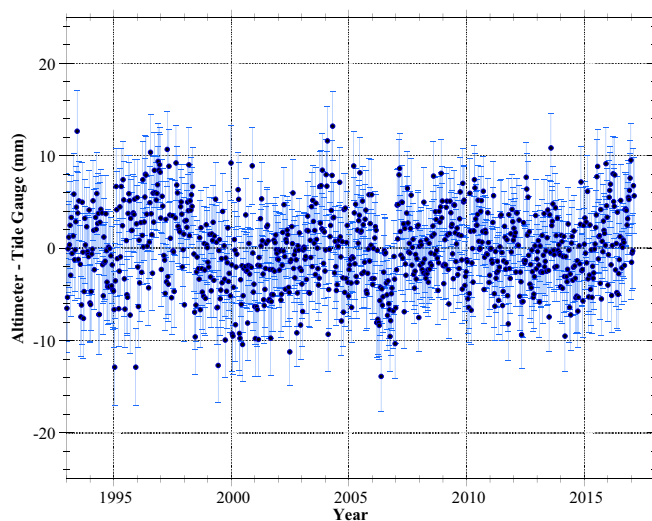
Fig. 3. Differences between altimeter and tide gauge observed sea level used to estimate the error in the acceleration estimate (13).
