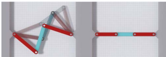
Fig. 5. Example of a triviar planar underconstrained mechanism. While the mechanism in Left has one degree of freedom, the mechanism in Right cannot move despite having the same number of constraints as the one in Left . For this reason, the mechanism in Right is designated as underconstrained.
