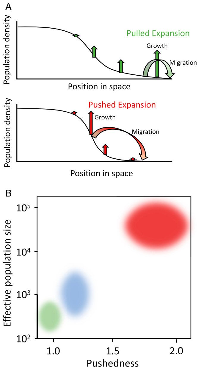
Fig. 1. Pushed versus pulled expansions lead to very different effective population sizes. (A) Pulled expansions have highest per capita growth rates at the leading edge and are pulled forward by a mixture of growth and migration at the leading edge. Pushed expansions have highest per capita growth rates at intermediate densities and are pushed forward by growth at intermediate densities spilling over via migration to fill in the leading edge. (B) Effective population size versus pushedness for spreading yeast populations grown on galactose (green), glucose (blue), and sucrose (red) solutions over a wide variety of experimental conditions (summarized and redrawn from ref. 8).
