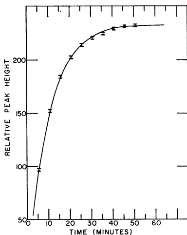
FIG. 2.—Typical plot of relative peak height versus time for the paramagnetic product P_2 arising from the deacylation of the spin-labeled \alpha -chymotrypsin, ES' (pH 6.8, 0.05 M phosphate buffer). Smooth curve represents theoretical first-order decay curve for k_3 = 1.6 \times 10^{-3} \text{ sec}^{-1} .
