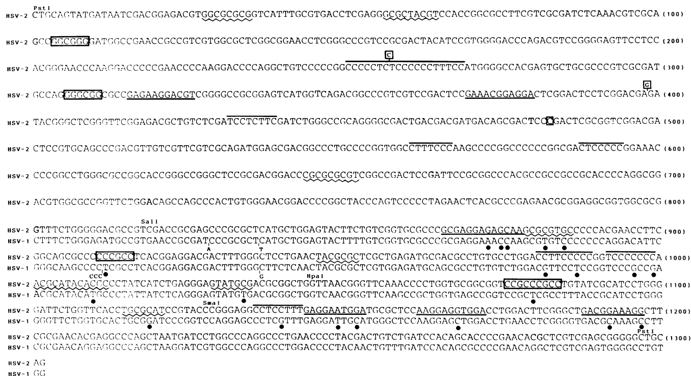
FIG. 3. Nucleotide sequence of the transforming HSV-2 domain and comparison with nontransforming HSV-1 DNA. The HSV-2 sequence presented is of the 1.3-kb Pst I-C region, in the prototypic orientation. Minimal transforming region extends from the Sal I to the Pst I site (nucleotides 822-1302). Single boxed nucleotides in HSV-2 DNA signify differences existing with the Swain and Galloway sequence (10). Four classes of repetitive elements are indicated: pyrimidine-rich (underlined), purine-rich (overlined), alternating purine/pyrimidine (zigzag underlined), and CCGCC sites (boxed). Base substitutions within repeats in HSV-1 DNA are shown by dots; the insertions are shown by vertical lines.
