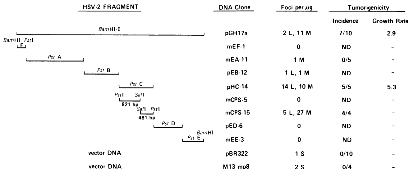
FIG. 2. Transforming potential of HSV-2 Bam HI-E subclones. Focus-formation data are the average of three experiments (focus size: L, large; M, medium; S, small). Tumorigenicity of isolated foci was assayed in syngeneic immunocompetent rats, and growth rate is expressed as \text{cm}^2/\text{week} . ND, analysis not done.
