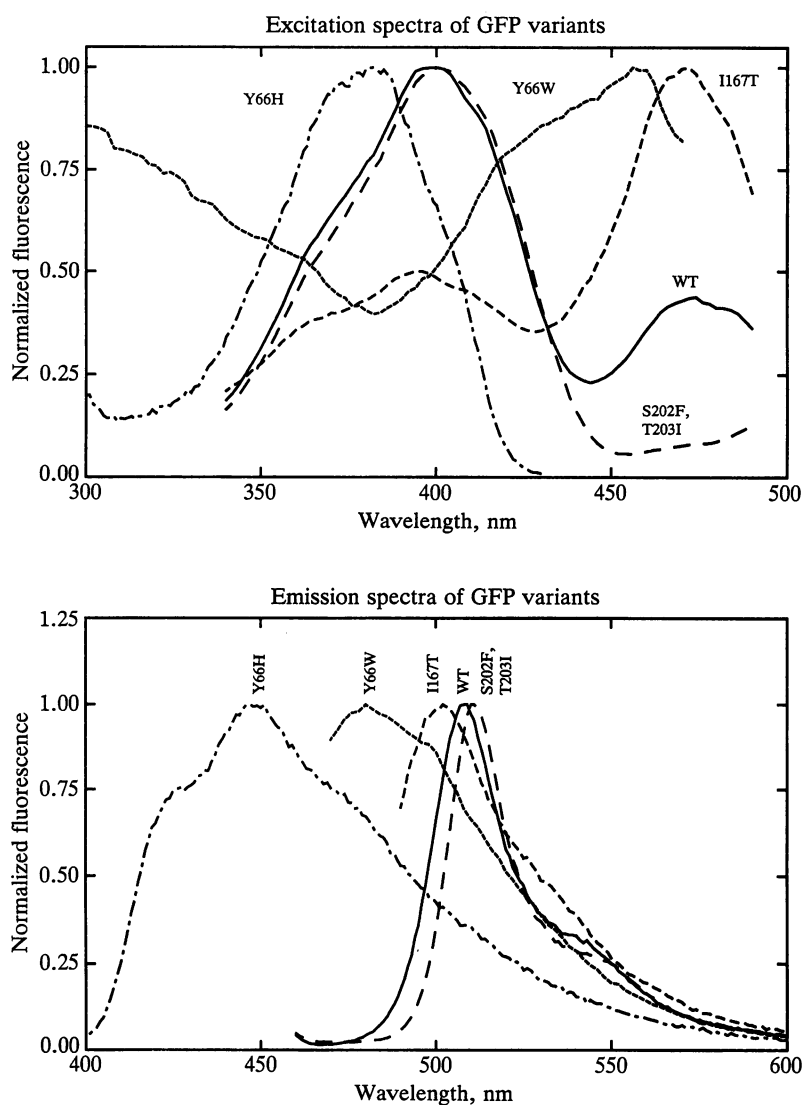
FIG. 3. Excitation and emission spectra of Wild-type and mutant GFPs. —, Wild-type; — —, mutations S202F, T203I; ---, mutation I167T; - - - -, mutation Y66W; — · —, mutation Y66H. Samples were soluble fractions from E. coli expressing the proteins at high level, except for mutant Y66W, which was obtained in very low yield and measured on intact cells. Autofluorescence was negligible for all spectra except those of mutant Y66W, whose excitation spectrum below 380 nm may be contaminated by autofluorescence. All amplitudes have been arbitrarily normalized to a maximum value of 1.0. To compare brightnesses at equal protein concentrations, see Table 1.
