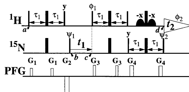
FIG. 1. Experimental scheme for TROSY-type two-dimensional ^1\text{H} , ^{15}\text{N} correlation spectroscopy. In the rows marked ^1\text{H} and ^{15}\text{N} , narrow and wide bars stand for nonselective 90^\circ and 180^\circ rf-pulses, respectively. Water suppression is achieved by WATERGATE (34), using the two off-resonance rf-pulses indicated by curved shapes. The ^1\text{H} and ^{15}\text{N} carrier frequencies are placed at 9 and 127 ppm, respectively. The delay \tau_1 corresponds to 1/(4J(^1\text{H}, ^{15}\text{N})) = 2.7 ms. Phases used are \psi_1 = \{y, -y, -x, x, y, -y, -x, x\} ; \psi_2 = \{4(x), 4(-x)\} ; \phi_1 = \{4(y), 4(-y)\} ; \phi_2 (receiver) = \{x, -x, -y, y, x, -x, y, -y\} ; x on all other pulses. The row marked PFG (pulsed field gradient) indicates the applied magnetic field gradients along the z -axis: G_1 , amplitude = 30 G/cm, duration = 0.4 ms; G_2 , -60 G/cm, 1 ms; G_3 , 50 G/cm, 0.4 ms; G_4 , 48 G/cm, 0.6 ms. Two free induction decays are recorded per t_1 delay, with \psi_1 incremented by 90^\circ in between and stored as the real and imaginary parts of the interferogram in t_1 . The Fourier transformation results in a two-dimensional ^1\text{H} , ^{15}\text{N} correlation spectrum that contains only the component of the four-line ^{15}\text{N} - ^1\text{H} multiplet that has the slowest T_2 relaxation rates for both nuclei. With this scheme, DD/CSA relaxation interference, which has been known for many years (35, 36), can be used to extend the limits of protein NMR.
