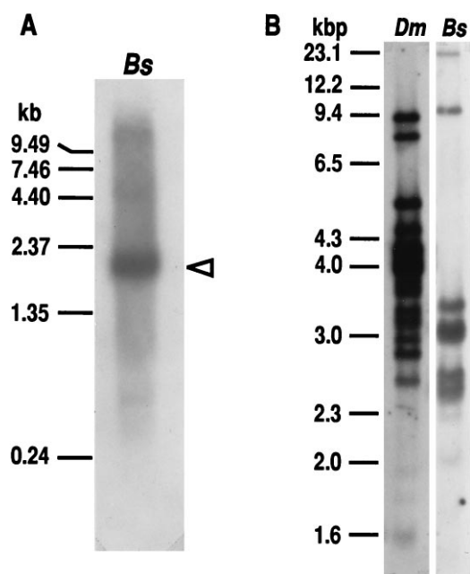
FIG. 4. (A) Northern blot of liver poly(A) + RNA from Arctic cod ( Bs ) showing multiple AFGP messages. \triangle , Predominant 1.8-kb mRNA. (B) Southern blot of genomic DNA digested with Mbo I from D. mawsoni ( Dm ) and B. saida ( Bs ) showing AFGP multigene family. Bracket indicates the range of DNA fragments recovered for construction of B. saida partial genomic library.
