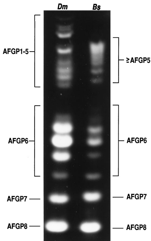
FIG. 1. Polyacrylamide gel of fluorescently labeled AFGPs from Antarctic nototheniid D. mawsoni ( Dm ) and Arctic cod B. saida ( Bs ) and the amino acid compositions of the three size groups of Arctic cod AFGPs. The two polar fishes show comparable size heterogeneity, especially in the range of AFGPs 6–8.
