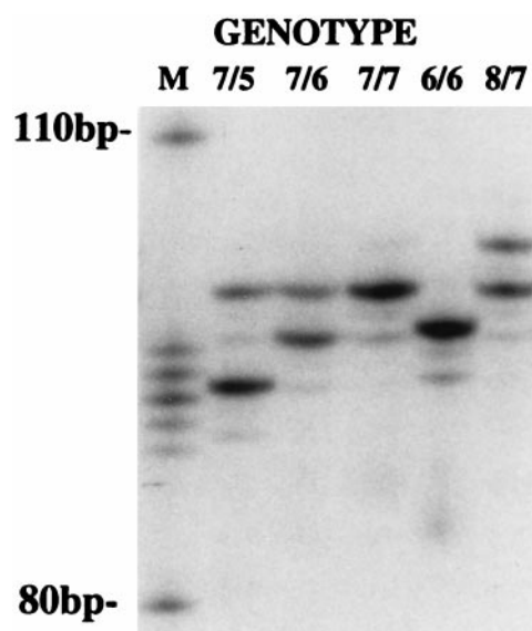
FIG. 1. Autoradiograph demonstrating the number of (ta) repeats in the UGT1A1 promoter. M denotes the SequaMark molecular weight marker ranging in size from 80 to 110 bp with 1-bp incremental bands in the center. DNA samples from subjects with (ta) 7 /(ta) 5 , (ta) 7 /(ta) 6 , (ta) 7 /(ta) 7 , (ta) 6 /(ta) 6 , and (ta) 8 /(ta) 7 UGT1A1 genotypes are shown. Method is described in the text.
